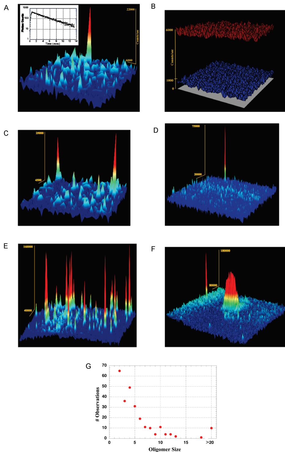
FIGURE 3: Examples of membrane-bound A \beta species. The panels show the fluorescence images (linear scale of counts per second) obtained by scanning the BLM surface with 460 nm excitation and monitoring through a 500 nm dichroic filter. The resolution in these 40 \mu m \times 40 \mu m scanned areas is near the diffraction limit ( \sim 0.5 \mu m). The emission intensity and fluorescence lifetime of an individual HL488 dye molecule are used to assess the number of fluorescently labeled A \beta molecules associated with discrete pores on the BLM surface. In the case of pores observed in this figure, the fluorescence lifetime has been within 10% of the lifetime of the free chromophore. On the basis of these numbers, we estimate that the structure on the BLM in panel A contains a single peak with two monomers and has a conductivity of <0.3 pS (i.e., below our detection limit). Rescanning of this surface indicated this peak exhibited a diffusion rate below the current measurement limit of 5 \times 10^{-4} \mu m 2 /s. (B) Nonconducting BLM surface with membrane-bound A \beta 40-HL488. The average fluorescence intensity corresponds to approximately four or five dye molecules per square micrometer of surface area (top red surface). The bottom surface (blue) shows the background from the BLM in the absence of labeled A \beta 40-HL488. (C) Two distinct, small, oligomers. On the basis of the lifetime-normalized fluorescence intensity, both most closely matched A \beta dimers. No membrane conductivity was detected. (D) Example of a single-membrane permeabilizing oligomer with a conductivity of 2 pS. The lifetime-normalized fluorescence intensity corresponds to that of an A \beta hexamer. (E) Several discrete structures are observed with a total conductivity of 80 pS, and the most intense fluorescence peaks correspond to structures with approximately 12–14 dye molecules. (F) At 250 nM labeled A \beta 40-HL488, extended and discrete structure coexist on the membrane. The total conductivity is 150 pS. (G) Histogram of 257 discrete species, including 103 species observed without corresponding conductivity data. The data at a size of 20 oligomers represent those of species with more than 20 peptides.
