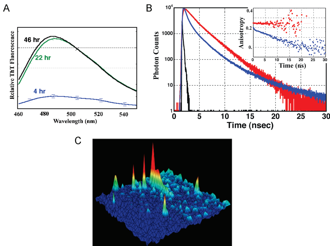
FIGURE 5: Interaction of A \beta with BLM followed by ThT binding. (A) Steady state fluorescence of 2 \mu M ThT (excitation at 440 nm) freshly added with A \beta 40 incubated for 4, 22, and 46 h at 37 ^{\circ} C in 10 mM sodium phosphate and 100 mM sodium chloride (pH 7.4). (B) Time-resolved fluorescence decay and time-resolved anisotropy of ThT added to A \beta after 4 h (blue) and 46 h (red) in solution. Excitation of ThT was at 425 nm, with emission monitored at 480 nm. The formation of A \beta fibrils is indicated by the large increase in the ThT fluorescence lifetime (and quantum yield) and the time-independent anisotropy decay reflecting a rotational correlation time in excess of the fluorescence decay window ( > 50 ns rotational correlation time). The ThT binding species at 4 h is best fit with a rotational correlation time of 15 ns. (C) ThT binding to unlabeled A \beta 40 on a 40 \mu m \times 40 \mu m BLM. Fresh A \beta 40 was incubated with the membrane for 10 min, and ThT (5 \mu M) was added. The conductivity of the BLM was 20 pS.
