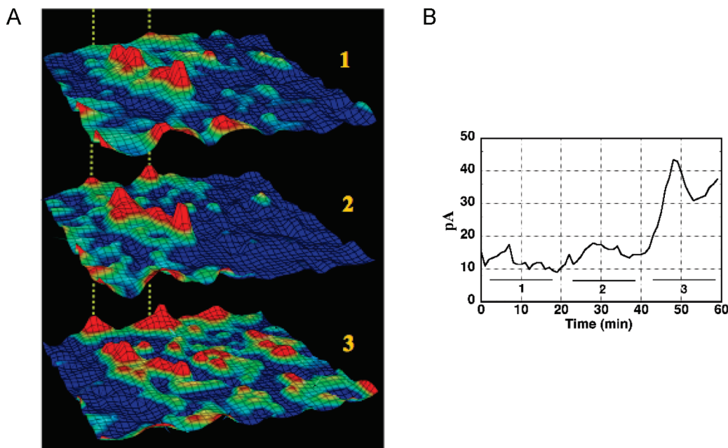
FIGURE 4: Time progression of extended pore structures. A \beta 40-HL488 (1 \mu M) was incubated with the BLM and formed extended pore structures that were dynamic in time. Raster scans of the 40 \mu m \times 40 \mu m BLM surface were initiated at approximately 1, 22, and 42 min (corresponding to solid lines labeled 1–3, respectively, in panel B) with a holding potential of 50 mV and show BLM surfaces with conductivities averaging (1) 230, (2) 280, and (3) 600 pS, respectively. The dashed lines in panel A indicate regions that underwent significant evolution in surface morphology. These membranes often disintegrate when the conductivity exceeds several nanosiemens for a 50 \mu m radius BLM. Since our resolution of conductivity is nominally 0.3 pS, the variation seen in panel B represents real changes in BLM conductivity. While some changes in fluorescence lifetime have been noted in the extended structures, it is not presently clear how much the intensity increase is associated with changes in the fluorescence quantum yield or increased concentration of labeled A \beta 40-HL488.
