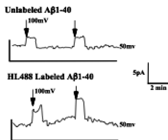
FIGURE 2: Conductivity plots for 100 nM unlabeled A \beta 40 and Hilyte 488-labeled A \beta 40 added to a BLM after a 4 h incubation in buffer at 20 °C. The BLM was maintained at a potential of 50 mV with transient changes to a potential of 100 mV (arrows).
